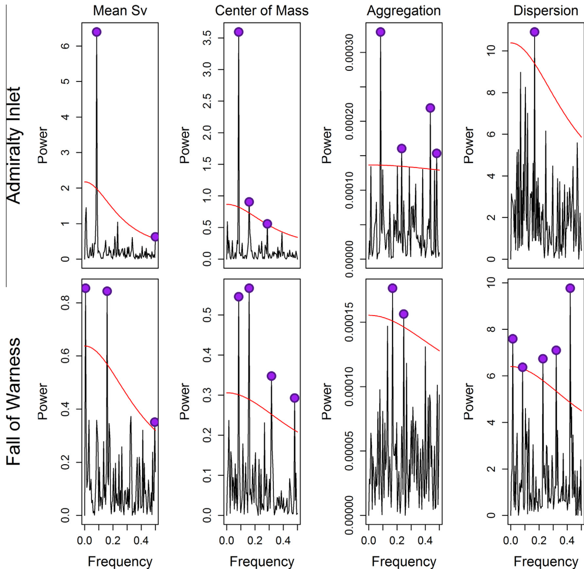
Fig. 7. Periodograms for the suite of metrics (mean S_v (dB), center of mass (m), dispersion ( m^2 ) aggregation ( m^{-1} )) at Admiralty Inlet and the Fall of Warness. Significant frequencies (purple dots) occur above the red noise spectrum (red line).
