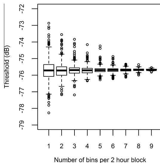
Fig. 3. Boxplots (0.95, 0.5, median) showing the distribution of threshold estimates for 500 draws from the Fall of Warness mean S_v (dB re 1 m -1 ) series containing 1 (10%) to 9 bins (90%) of the data.
